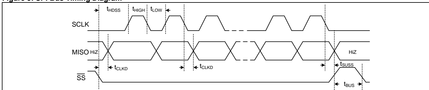
Figure 3: SPI Bus Timing Diagram
