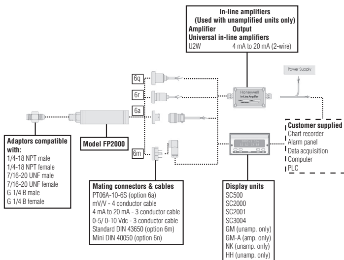
FIGURE 1. TYPICAL SYSTEM DIAGRAM
