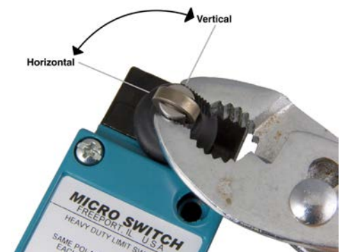
Figure 6. Top roller plunger adjustment
