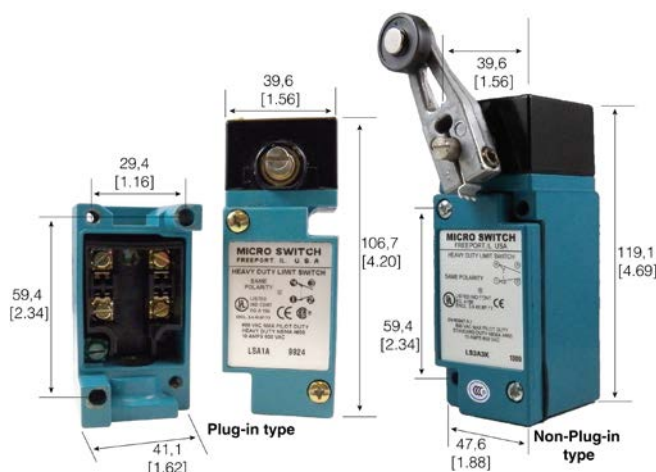
Figure 1. MICRO SWITCH™ HDLS SPDT Dimensions
