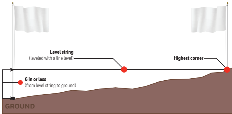
Figure 1. Grade Measuring
