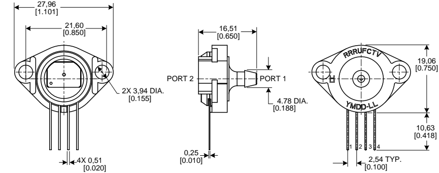
Figure 3. SIP Package Dimensional Drawings (continued)
