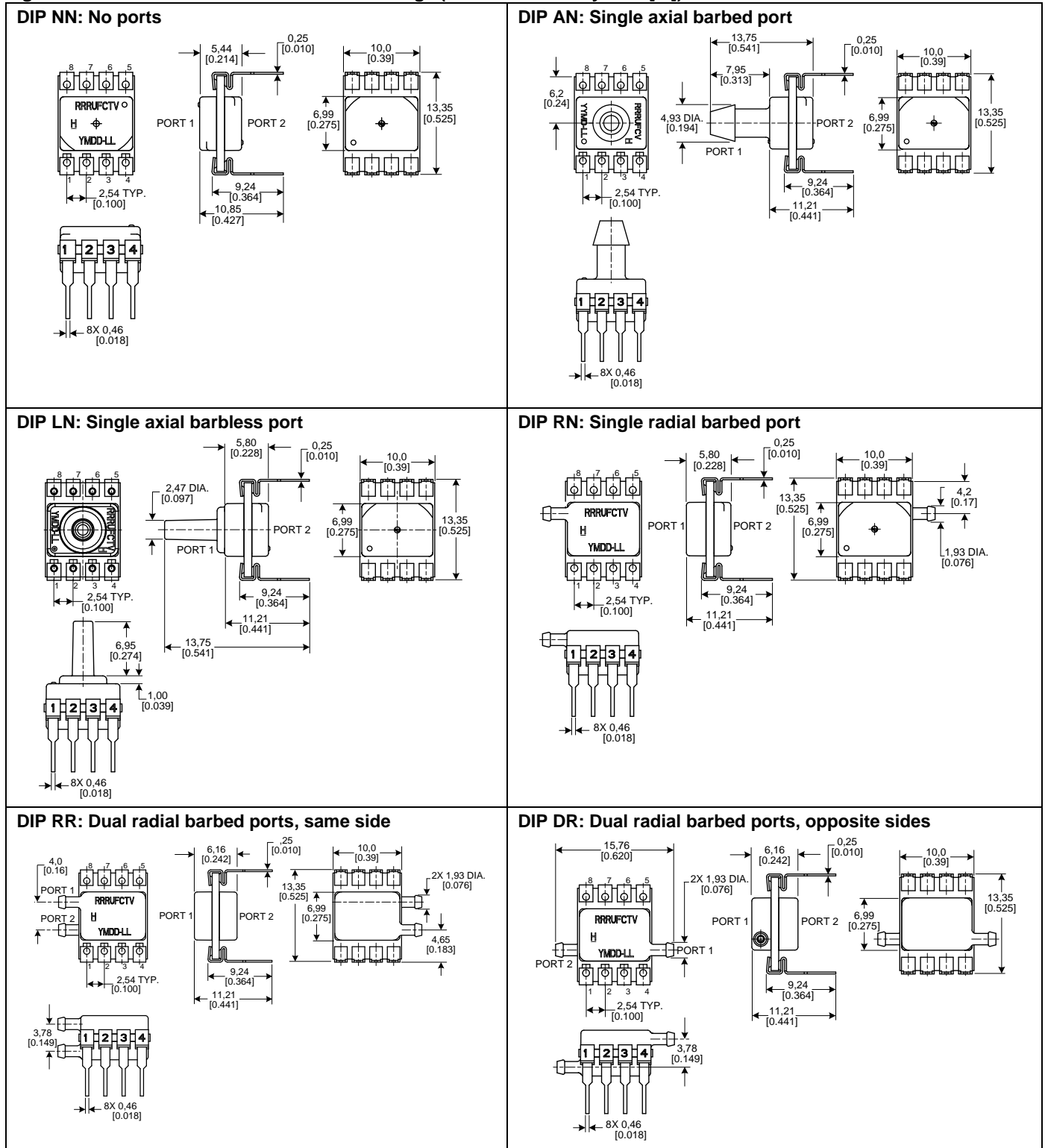
Figure 1. DIP Pressure Port Dimensional Drawings (For reference only: mm [in])
